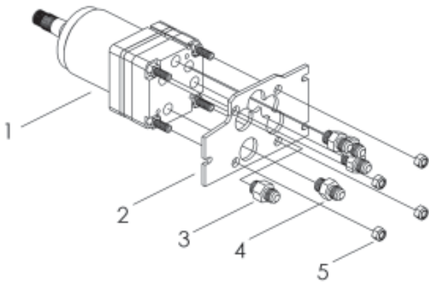
STEERING ORBITAL SUB-ASSEMBLY
