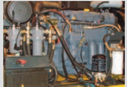
The engine: Rear, transverse positioned for ease of access and maintenance.
