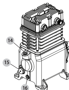
Compressor Pump
