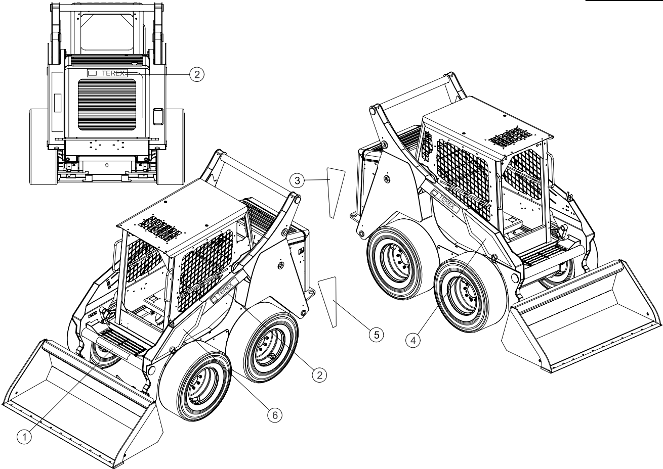
Decal Kit: 7006-213
