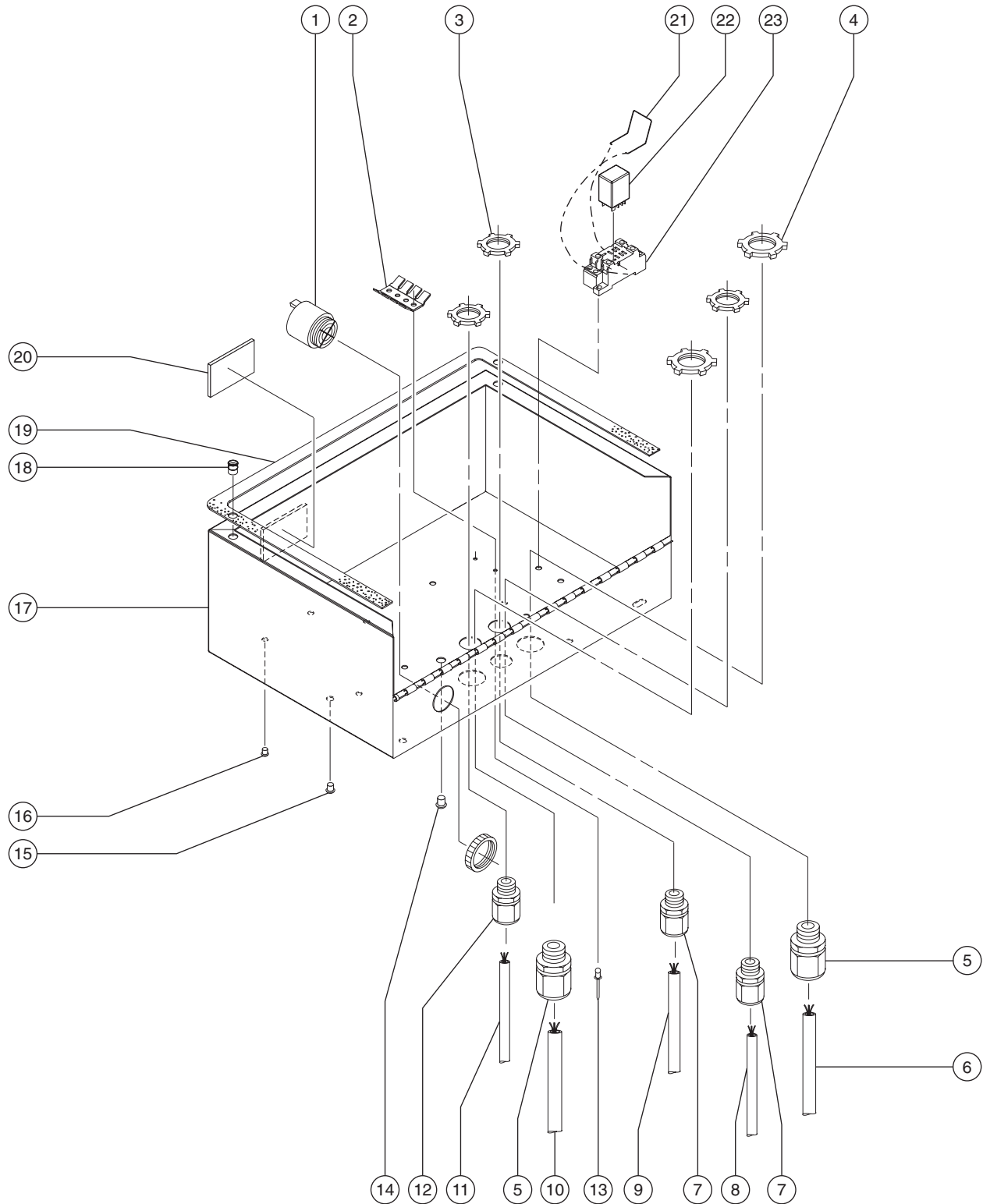
Figure Rev Description 606.1 B Platform Control Box - View 1 (after serial number 2750, Z-34/22N and 1999, Z-34/22DC)
