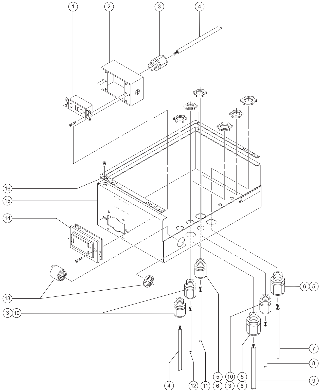
Figure Rev Description 604.1 B Platform Control Box - View 1(before serial number 2751, Z-34/22N and 2000, Z-34/22DC & Bi-Energy)
