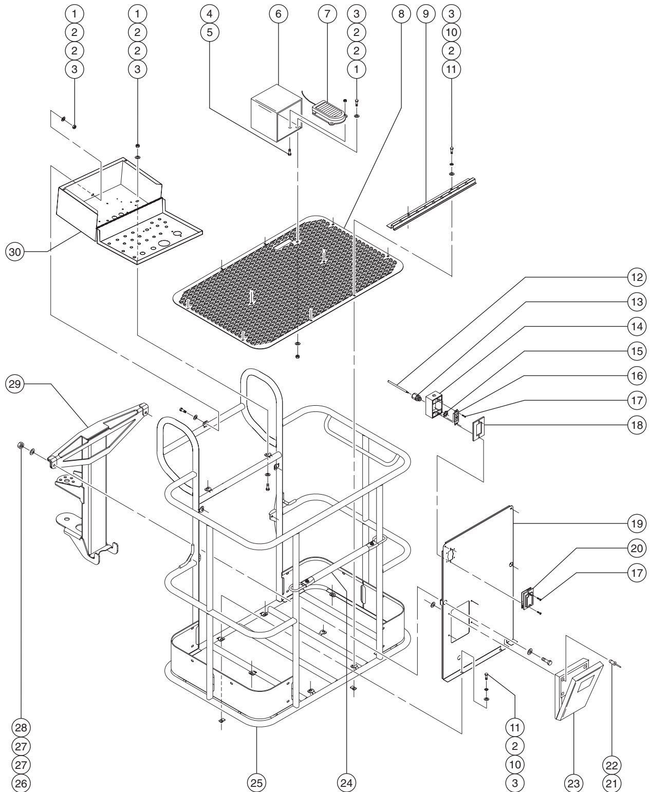
Figure Rev Description 602.1 A Platform (from serial number 2548 to 4259, Z-34/22N and 1892 to 3576, Z-34/22DC & Bi-Energy)
