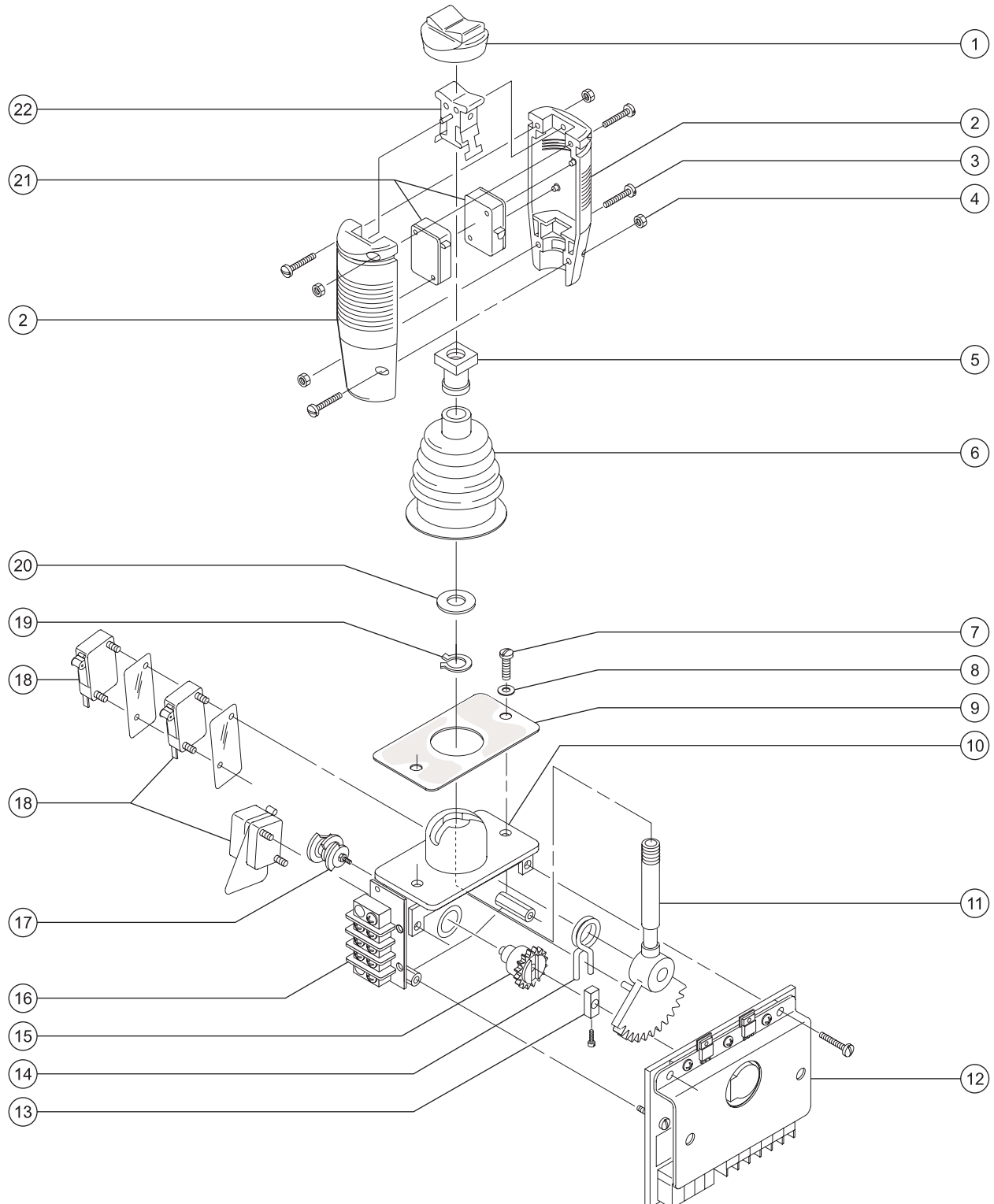
Figure Rev Description 608.1 B Joystick Controller - Drive/Steer Functions (before serial number 2227, Z-34-22N and 1734, Z-34/22DC & Bi-Energy)
