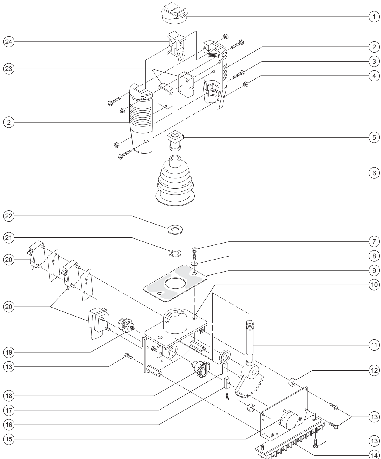
Figure Rev Description 609.1 A Joystick Controller - Drive/Steer Functions (after serial number 2266, Z-34/22N and 1733, Z-34/22DC & Bi-Energy)
