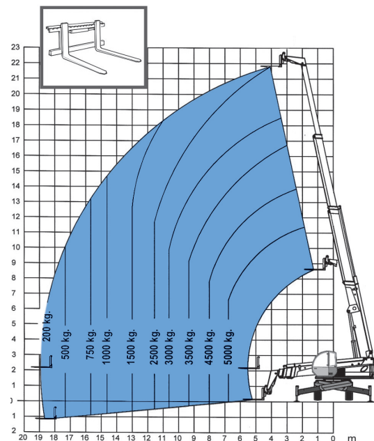
Lift capacity chart (with stabilisers)
