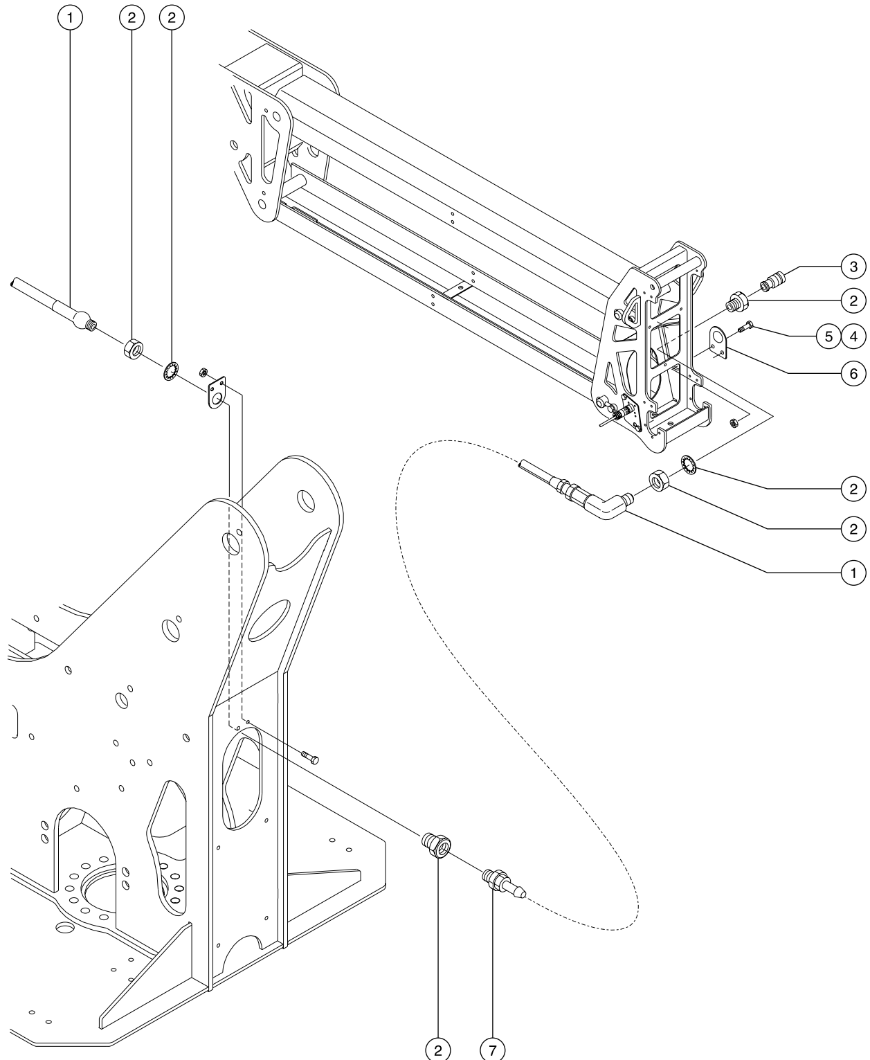
Figure 6-D Air line to Platform
