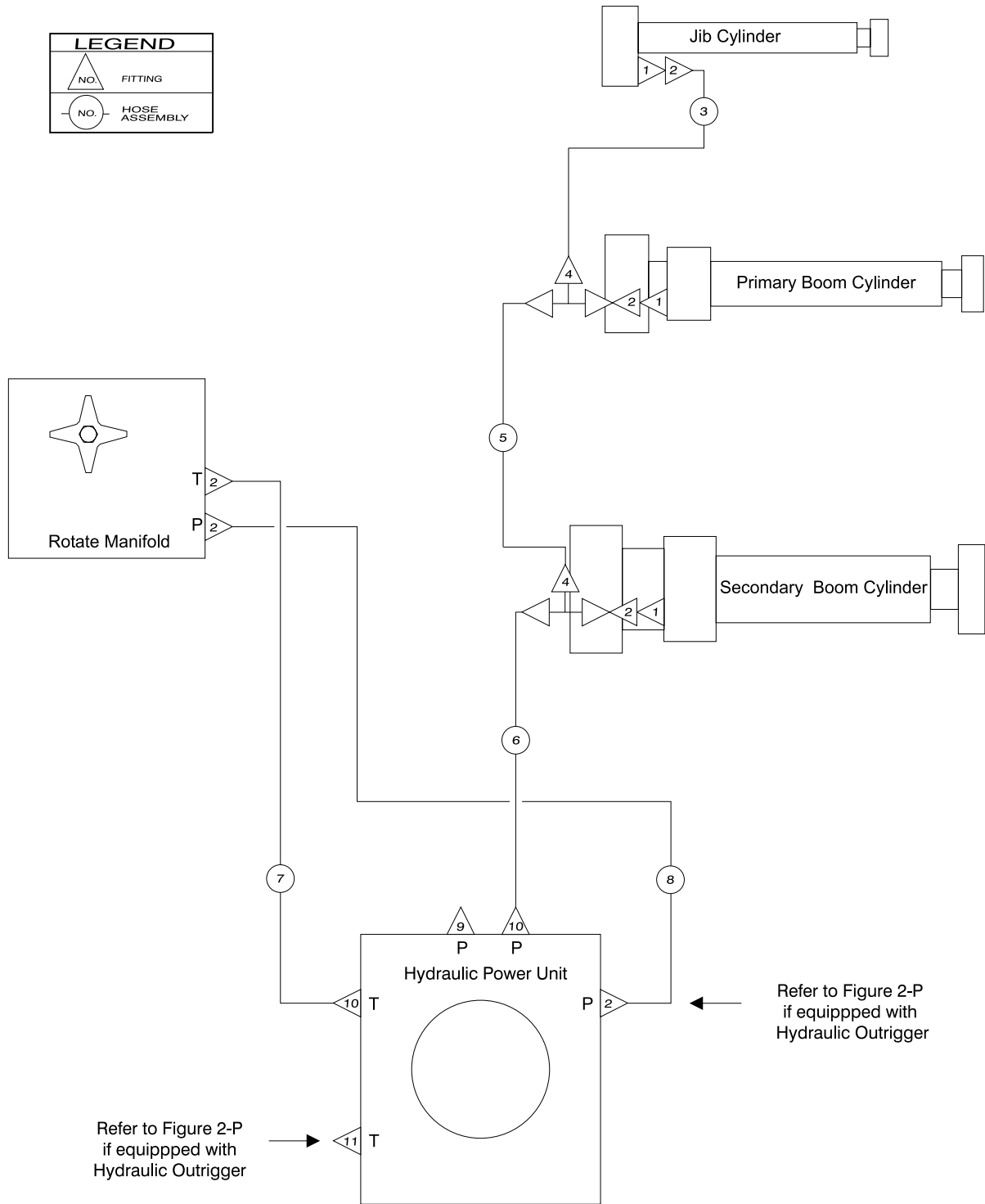
Figure 3-J Hydraulic Hoses and Fittings
