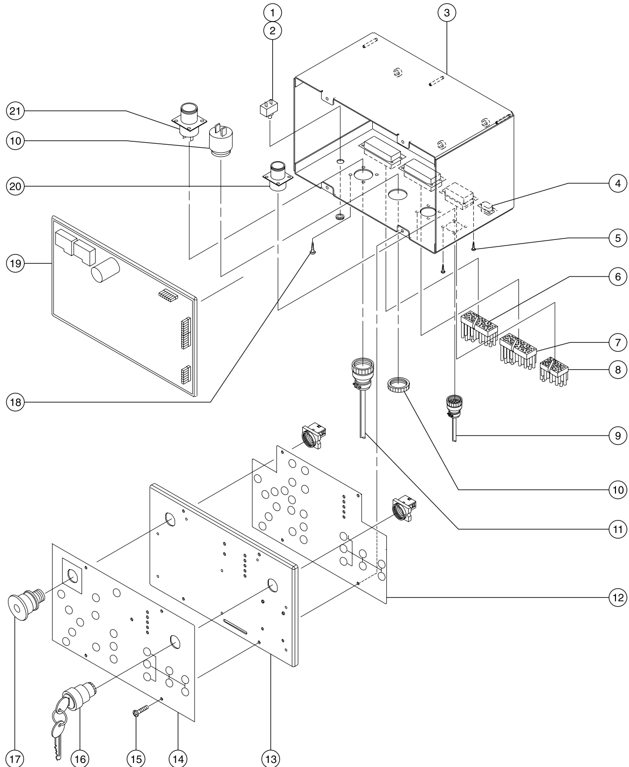
Figure 3-D Ground Controls
