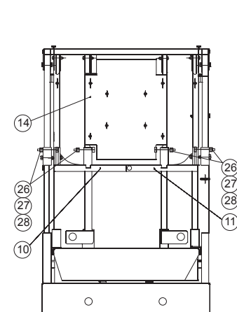
H - H
