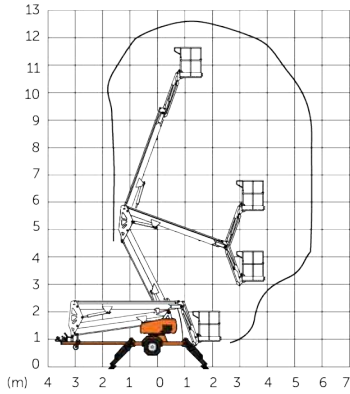
▶ Snorkel MHP 13
