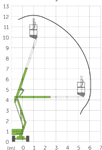
Nifty HR12
