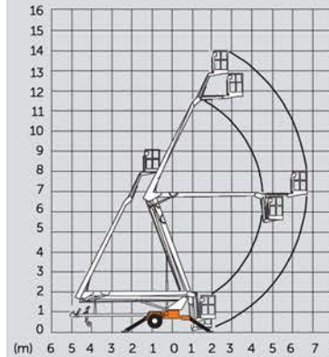
▶ Snorkel MHP 15
