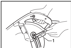
1. Lock lever
