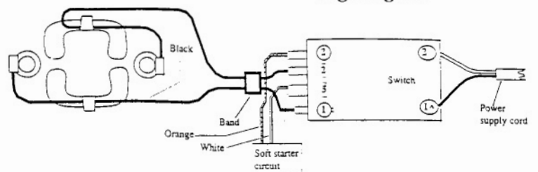
Wiring Diagram
