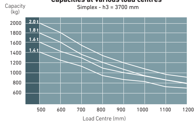
Capacities at various load centres
