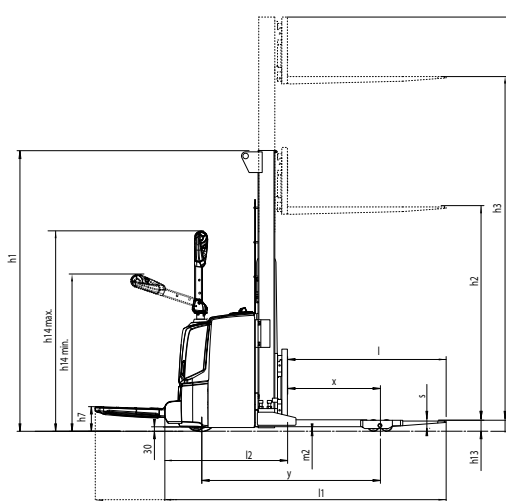
SBP16N3SR WIDE STRADDLE WITH FOLDING PLATFORM
