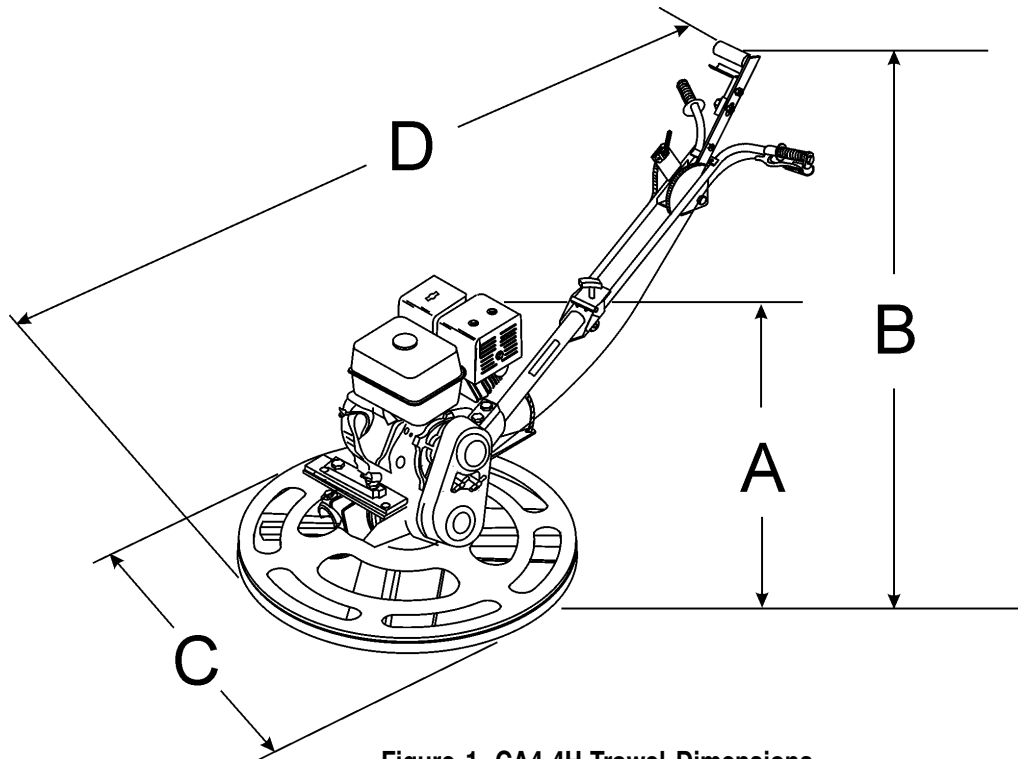
Figure 1. CA4-4H Trowel Dimensions
