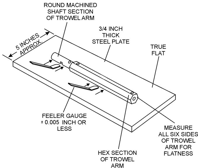
Figure 27. Trowel Arm Flatness Test
