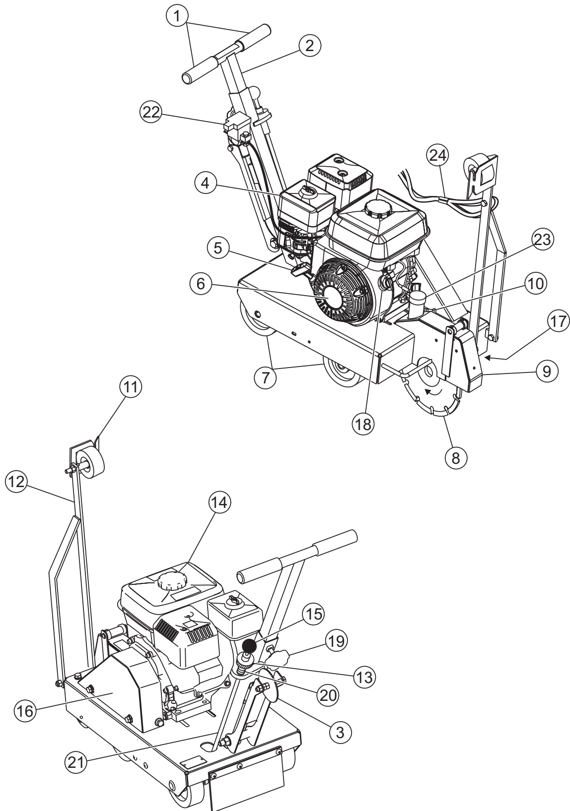
Figure 3. SFCG1 Concrete Saw
