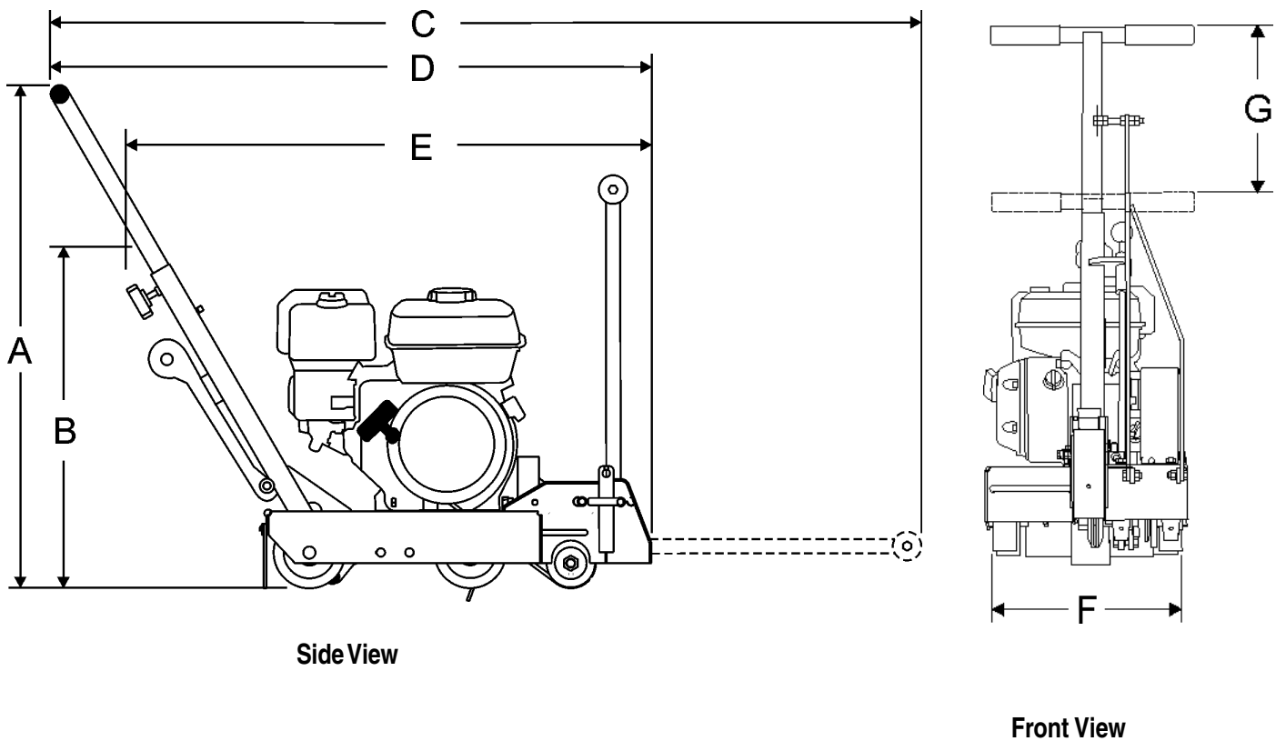
Figure 1. SFCG1 Concrete Saw Dimensions
