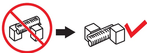
Figure 2. Rebar Placement
