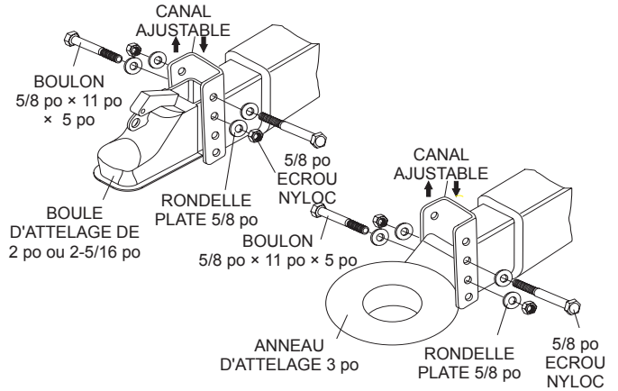
Figure 66. Canal ajustable
