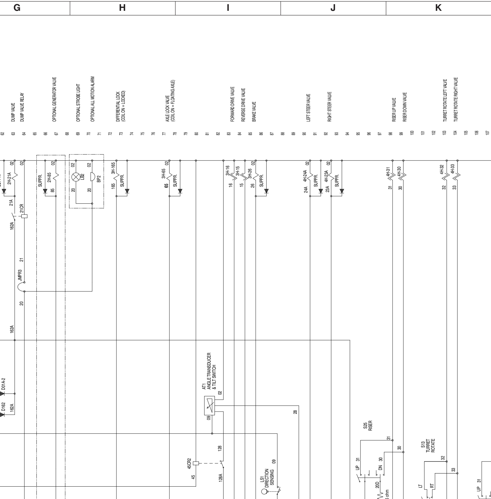
Electrical Schematic Diagram (CE SJ 46AJ/51AJ - Deutz Diesel Engine)
