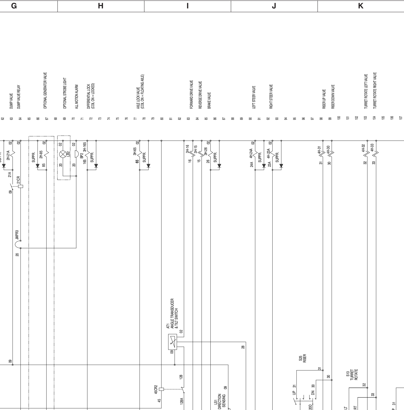
Electrical Schematic Diagram (ANSI/CSA SJ 46A/46AJ - GM Dual Fuel Engine)
