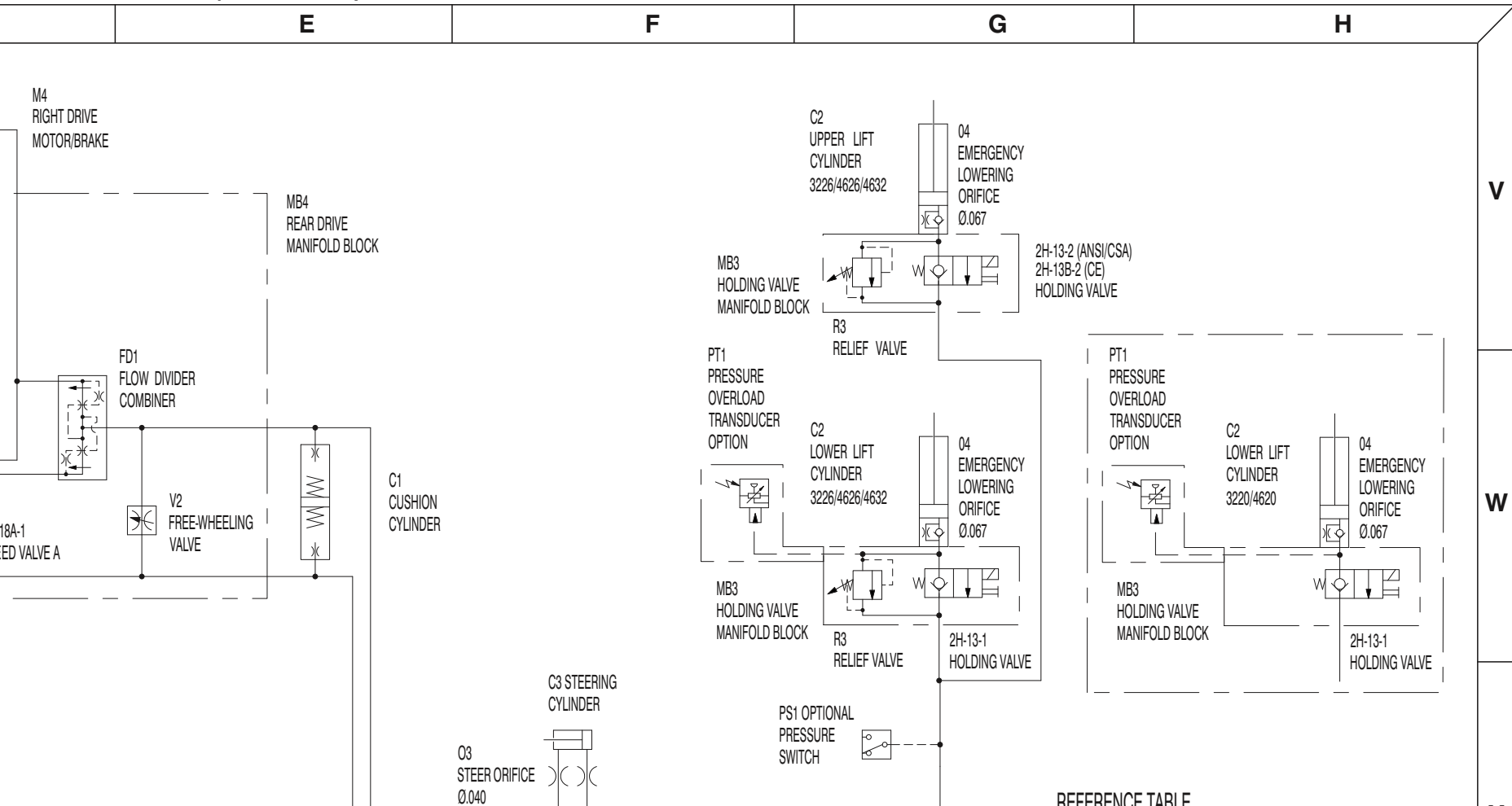
Hydraulic Schematic (Model 46xx)
