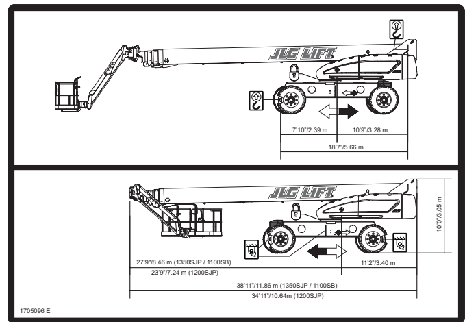
1705096 Lift Diagram (1200/1350)
