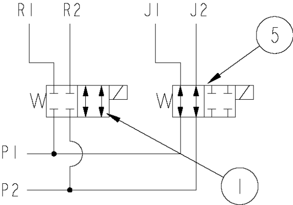
HYDRAULIC SCHEMATIC
