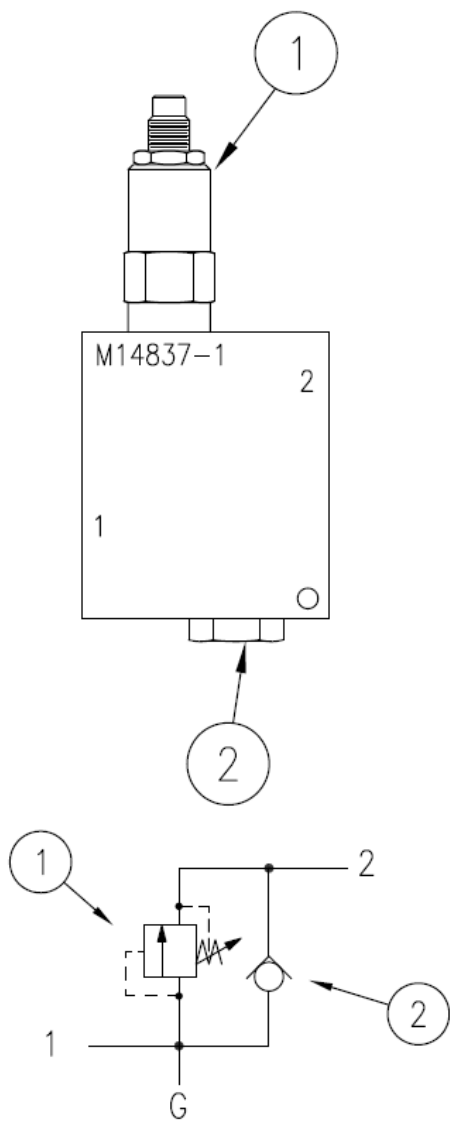
HYDRAULIC SCHEMATIC
